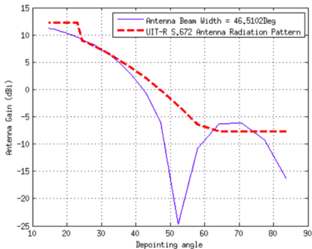
Fig. 10. Helical antenna radiation pattern.
