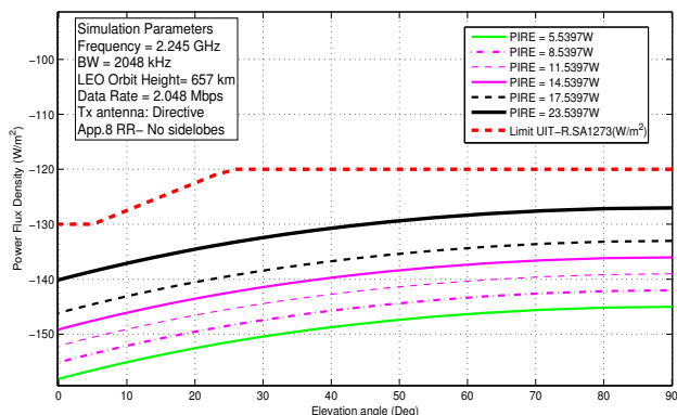
Fig. 8. Power flux density over the Earth (Omnidirectional pattern).
